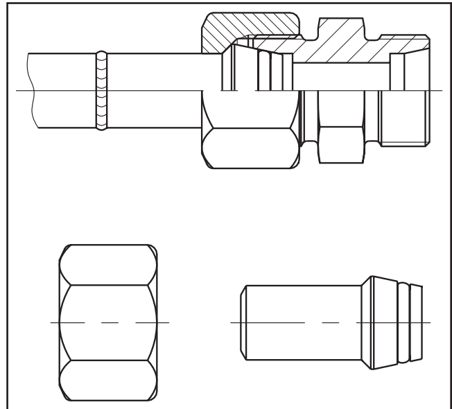
EO-Weld Nipples
