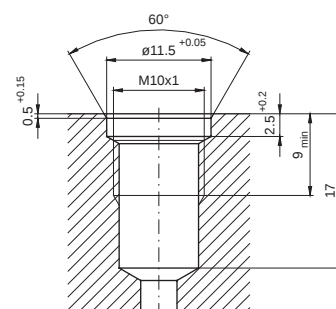
Screw-in hole M10x1/OR
